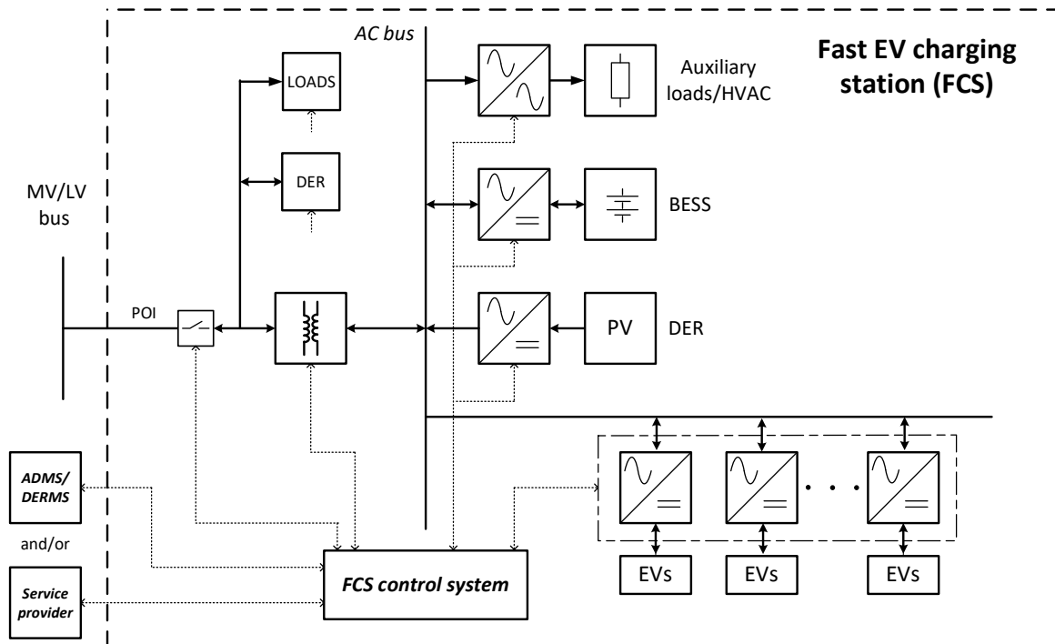
Figure B.2—Generic FCS Configuration and Assets—Local AC Bus 1
