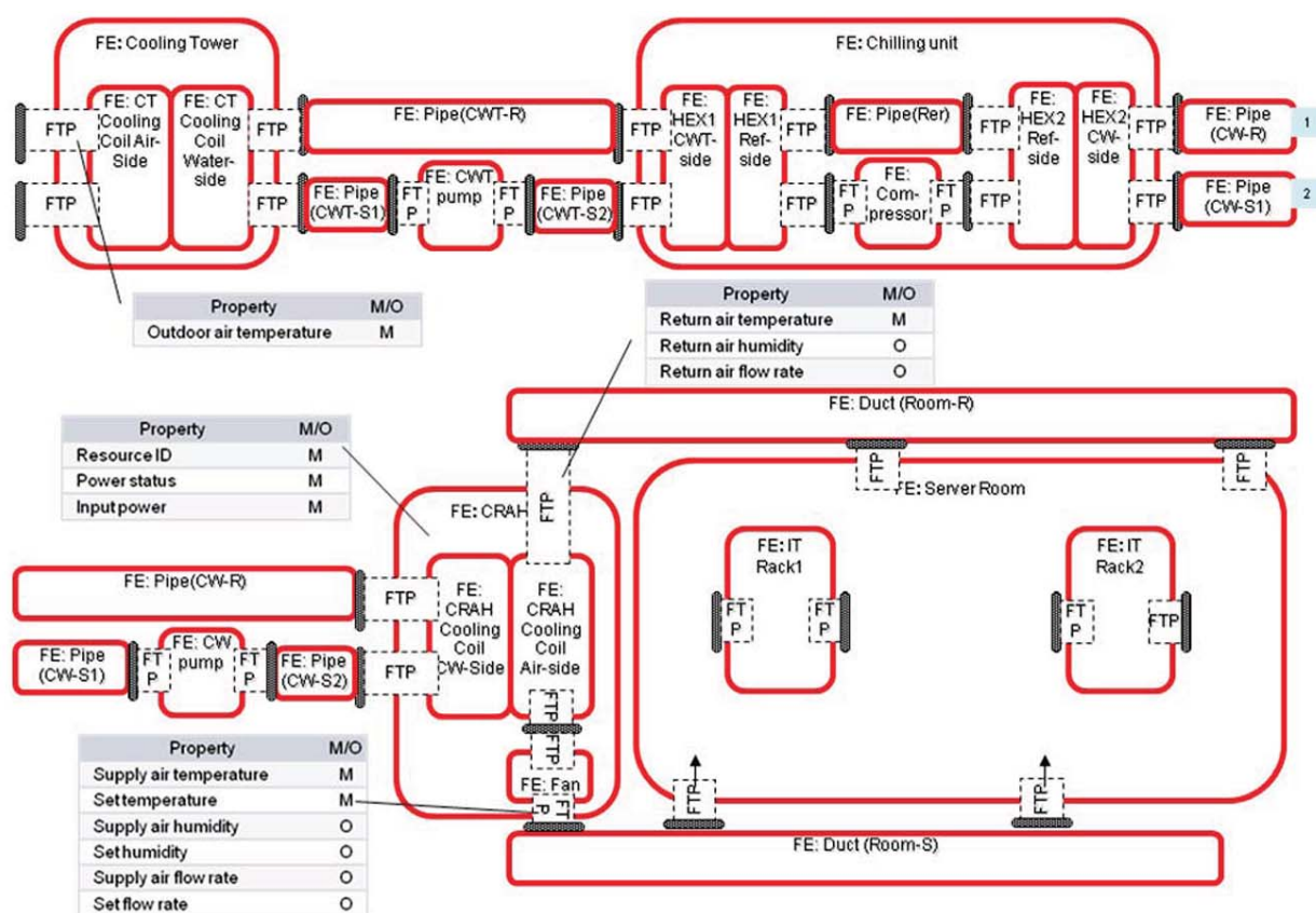
Figure B.1 — Fluid perspective representation of CRAH system
